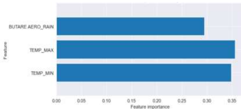
Figure 19: Features-Selection (Huye)
