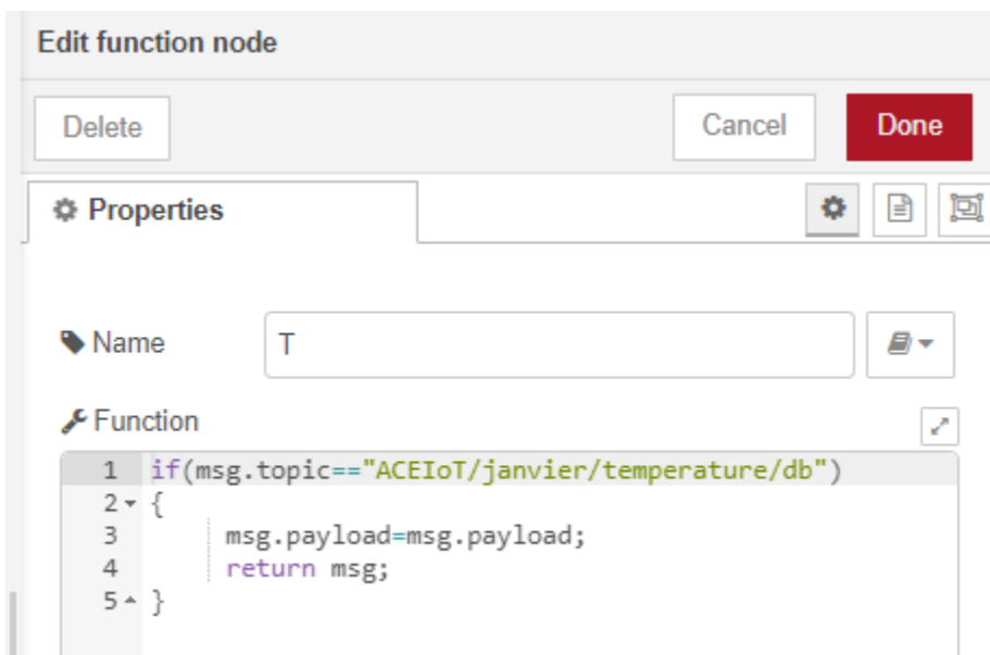
Figure 32: Node-Red-Function Implementation
