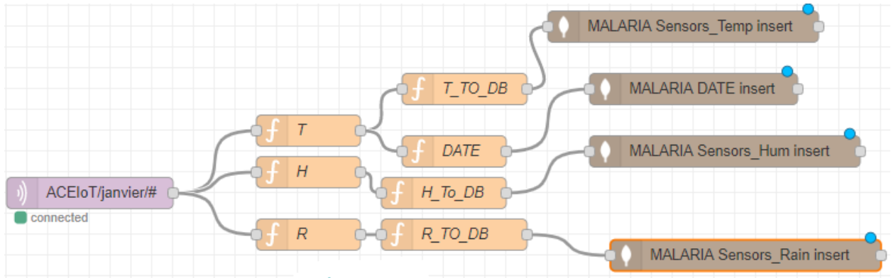
Figure 29: MQTT-Node-Red-Database Communication
