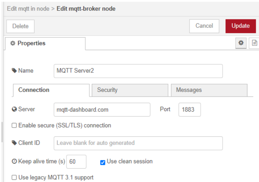
Figure 31: Node-Red-MQTT-Node-configuration
