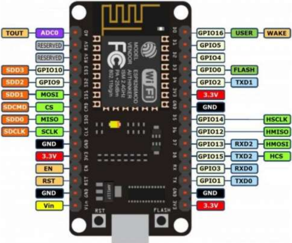
Figure 26: NodeMCU
