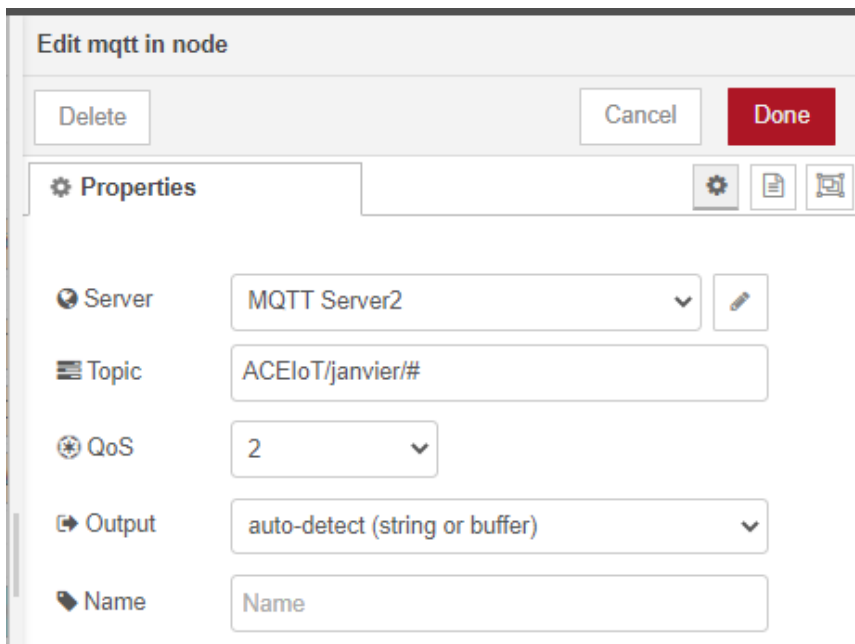
Figure 30: Node-Red-MQTT-Node implementation
