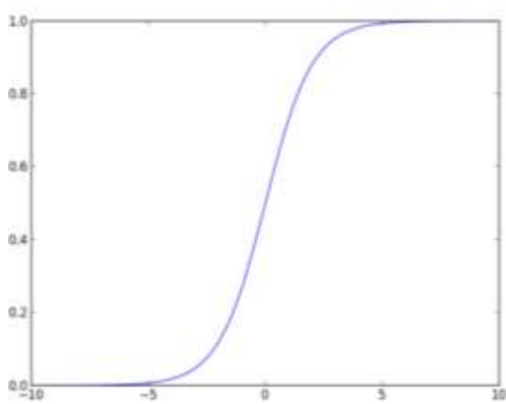
Figure 12: Sigmoid function
