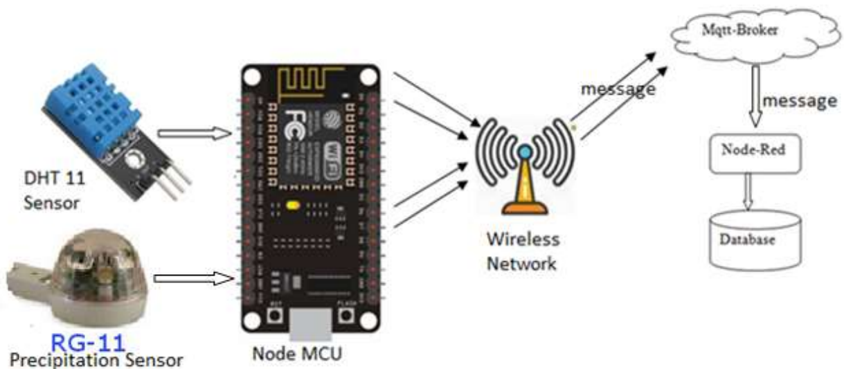
Figure 28: Wireless Communication system
