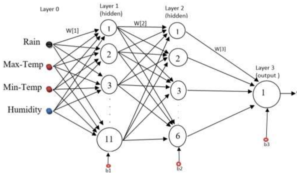
Figure 17: Artificial Neural Network architecture
