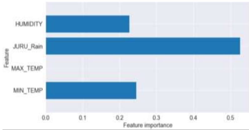
Figure 18: Features-Selection (Bugesera)
