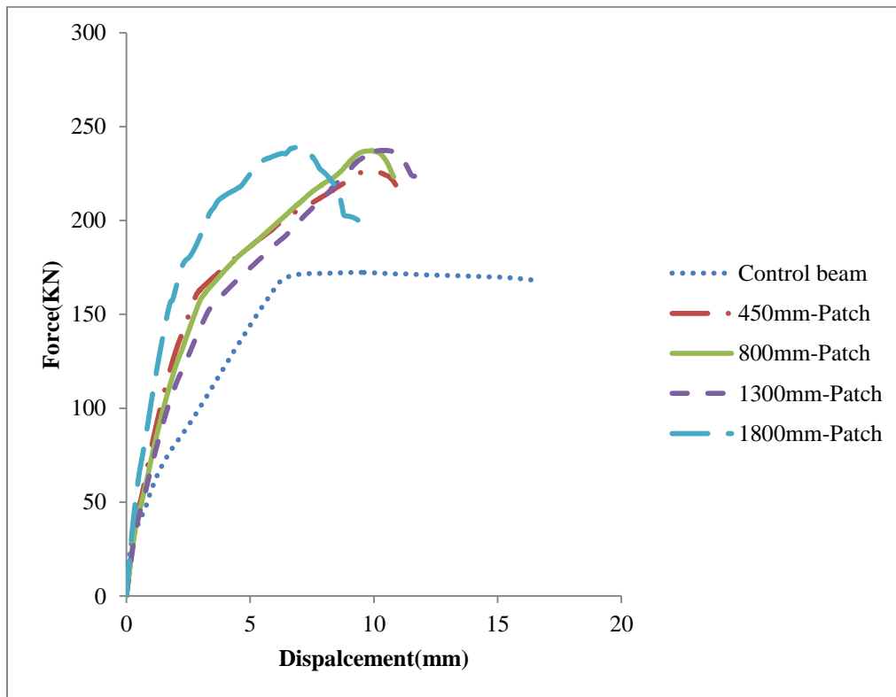
Figure 5.15: Load deflection relationships for all specimens.
