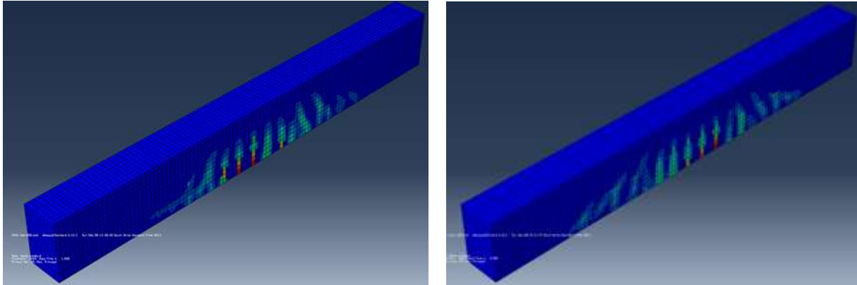
Figure 5.8: Crack distribution: 800mm-Patch (left), 1300mm-Patch (right).
