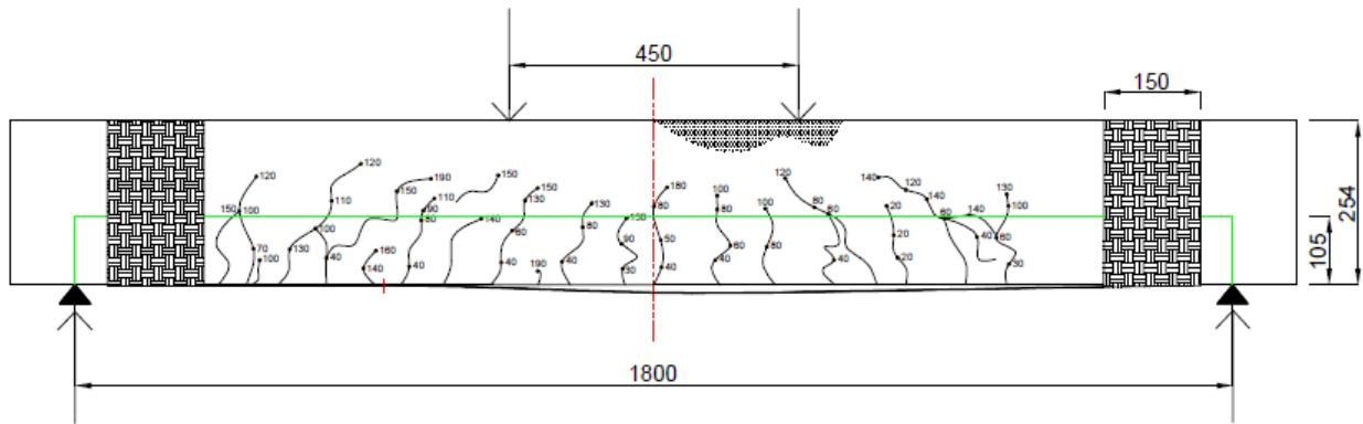
Figure 5.33: Structural rack pattern for 1800mm-Patched beam: Experiments.
