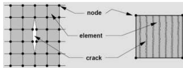
Figure3.14: Crack approaches: Discrete (left), Smearred (right) (Kwak &Filippou, 1990:25).
