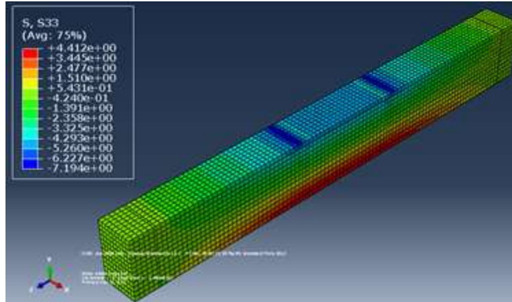
Figure 5.2: Tensile stress distribution in 1800mm-Patch repaired RC beam.
