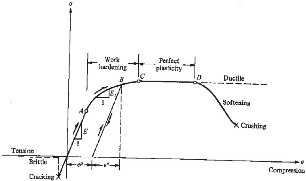
Figure 3.5: Uniaxial stress strain curve, pre and postfailure regime (Chen, 1982).
