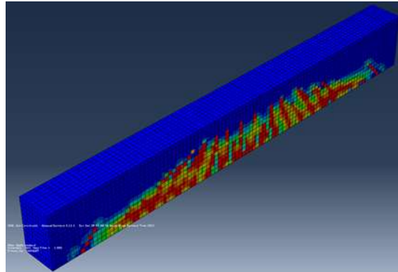
Figure 5.11: Tensile damage for control beam
