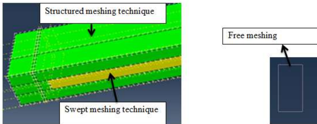
Figure 4.13: Meshing techniques.
