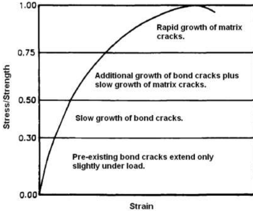
Figure 3.1: The compressive stress-strain curve for concrete
