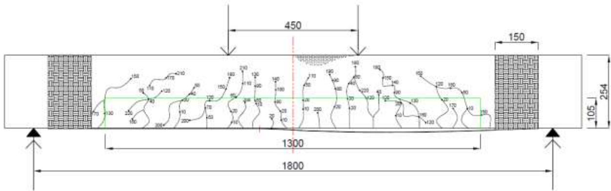
Figure 5.27: Structural rack pattern for 1300mm-Patched beam: Experiments.
