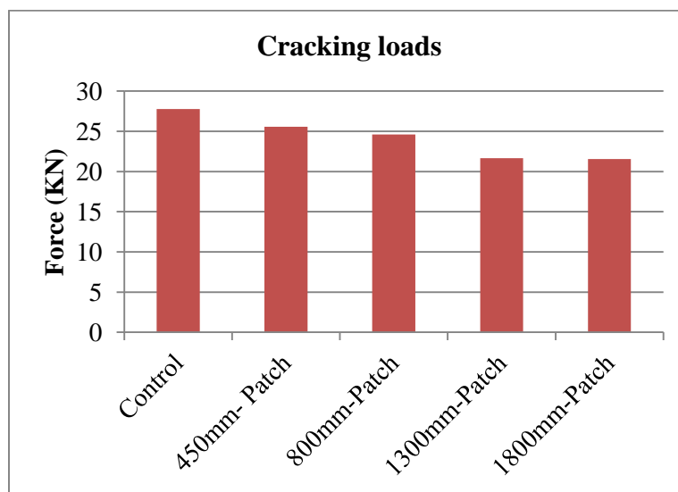
Figure 5.3: Cracking loads
