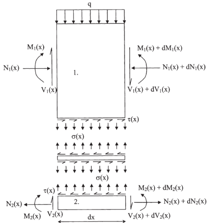
Figure 2.8: Interfacial shear and normal stress distribution (Smith and Teng, 2001)
