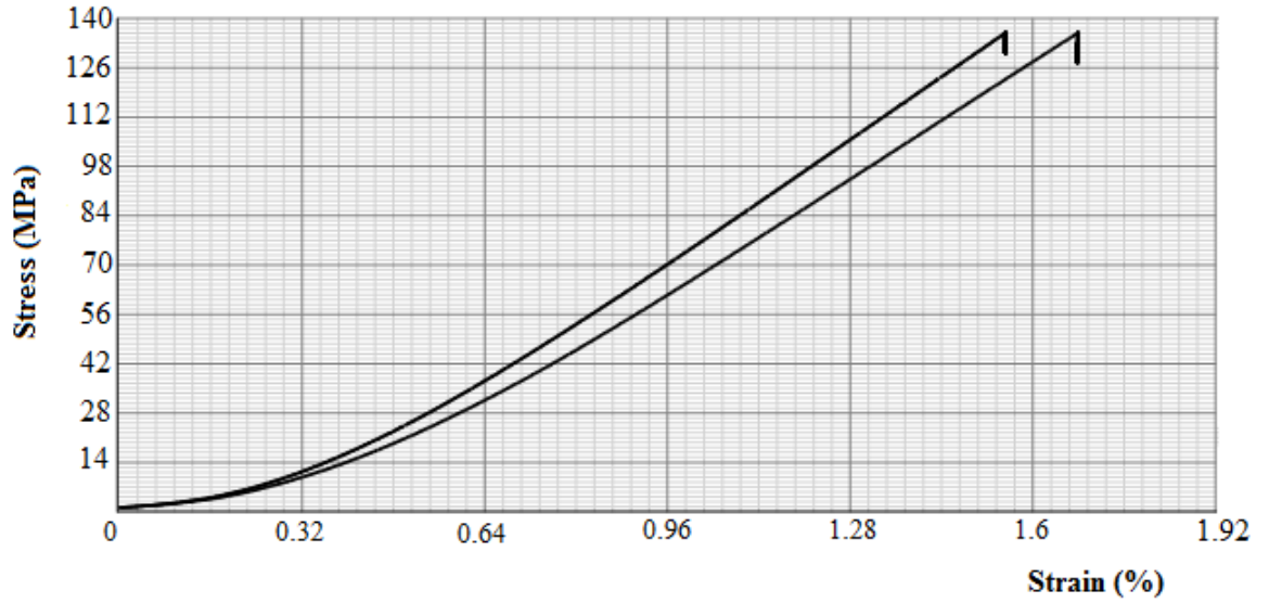
Figure 4.15: Compression test stress-strain curves
