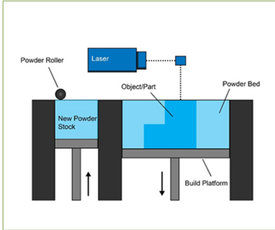
Figure 2.5: Principle of powder bed fusion process
