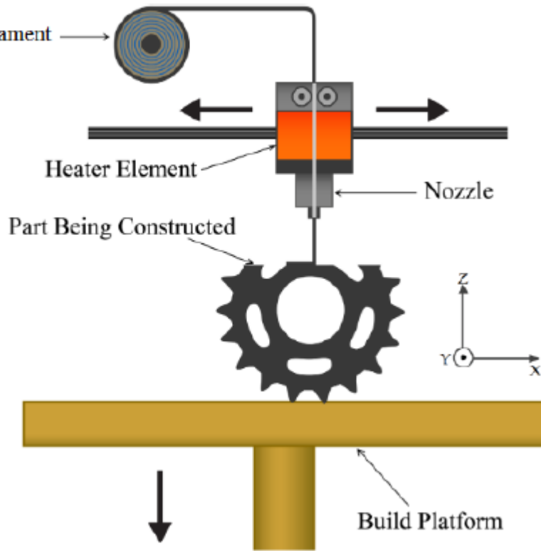
Figure 2.4: Principle of extrusion process
