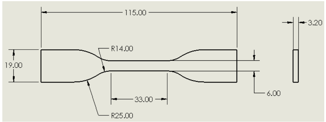
Figure 3.13: Dimension of tensile test specimen (mm).
