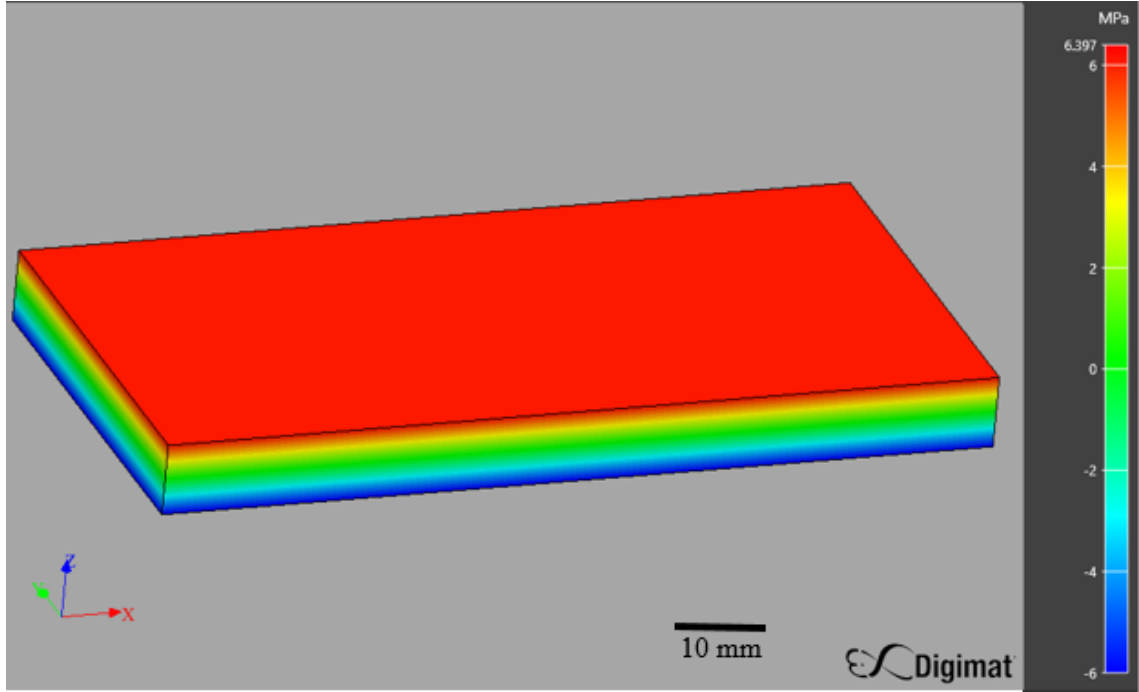
Figure 4.1: Preliminary residual stress results
