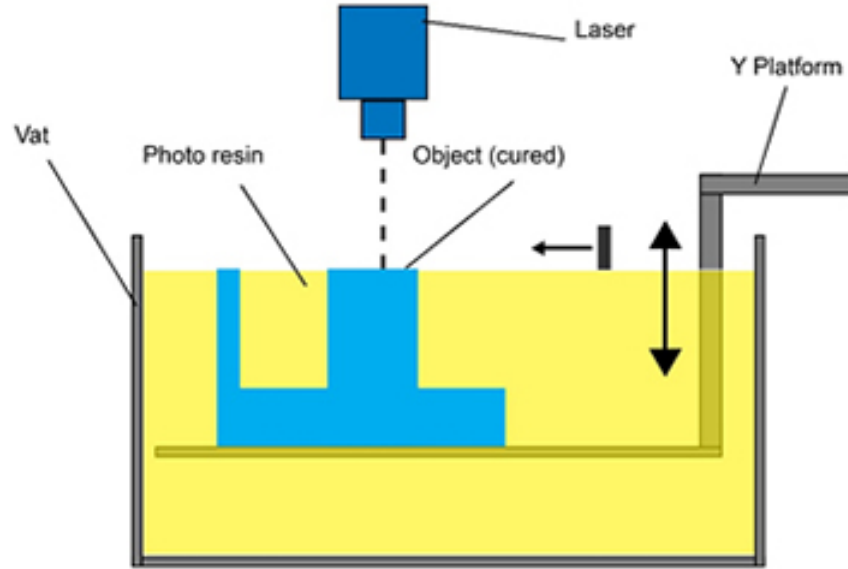
Figure 2.1: Principle of vat photopolymer (Dancel, 2019; Monzón et al., 2017)
